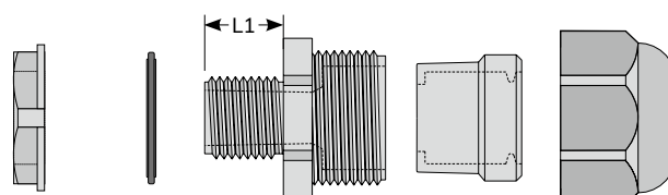
Part No.: Lock Nut BML, Washer BMW, Body BMB, Seal BMS, Nut BMN
